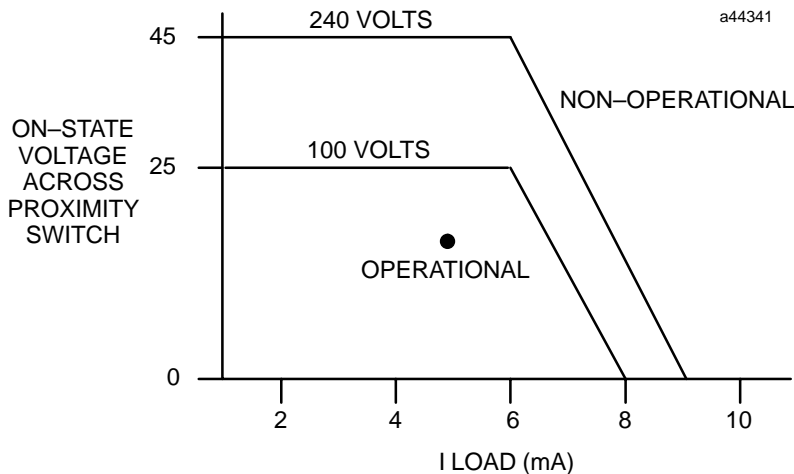
Figure 2. On-State Characteristics Compatibility
