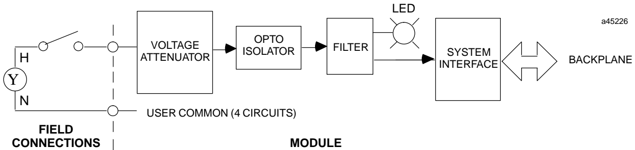
Figure 1. Block Diagram for IC697MDL251
