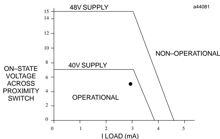
Figure 2. Proximity Switch Compatibility
