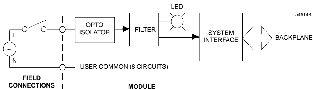
Figure 1. Block Diagram for IC697MDL254
