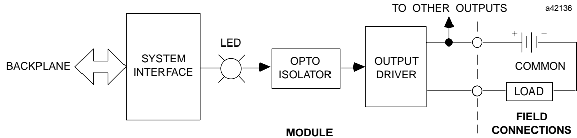
Figure 1. Block Diagram for IC697MDL752
